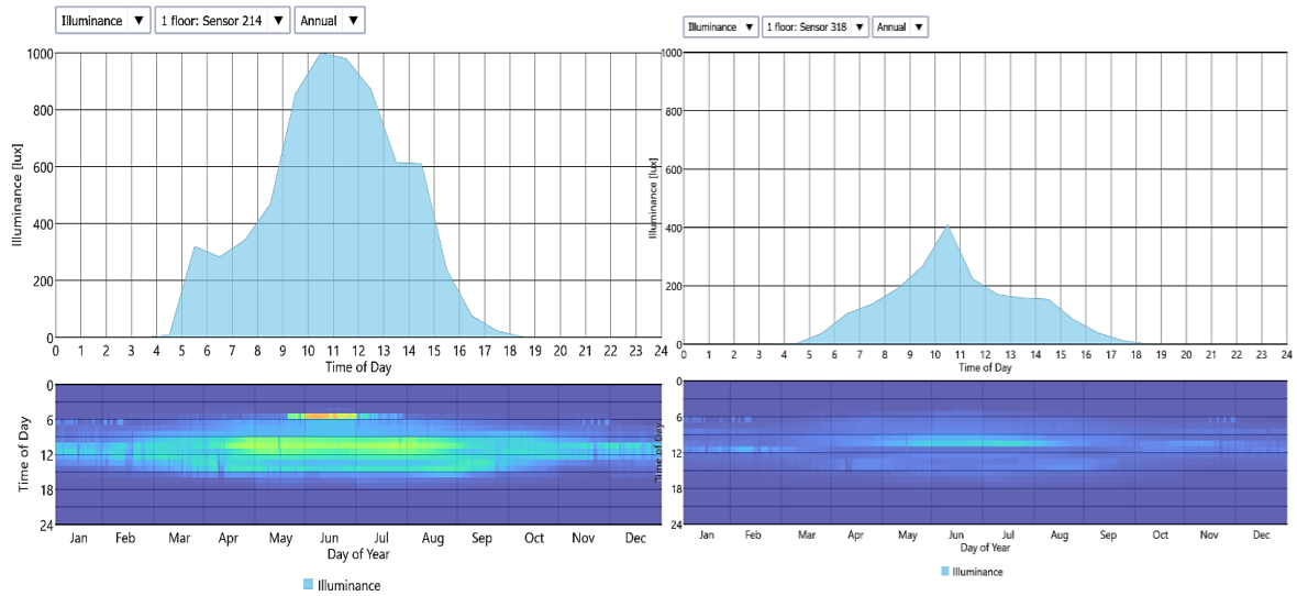
Figure 20 A graph showing the difference between the light intensity levels during the year for the library before and after installing SolaTube in areas where the intensity of illumination is below the required limit.
