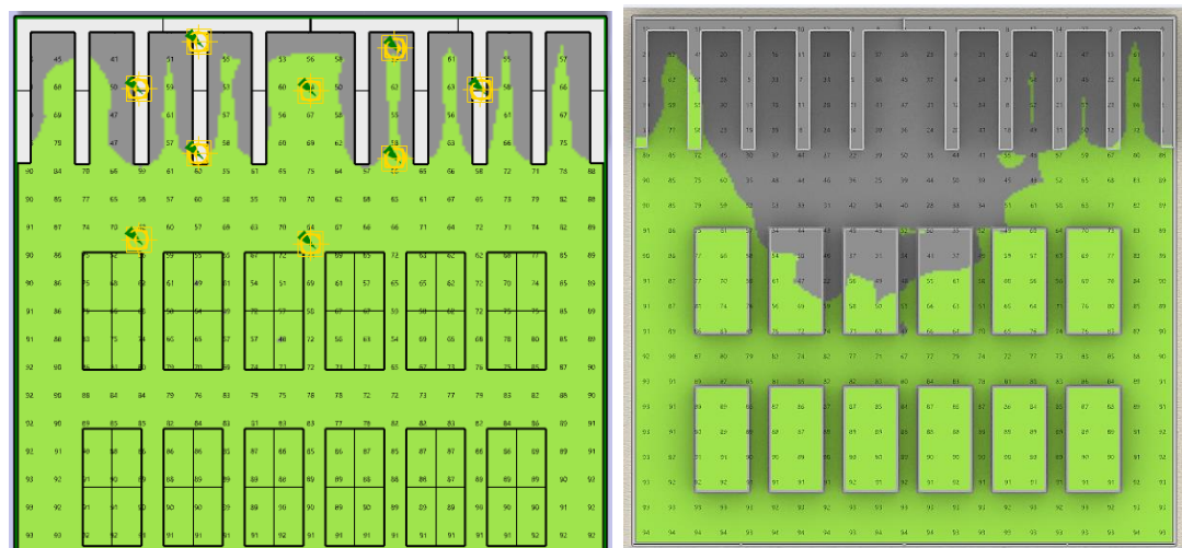
Figure 21 Measurements of the amount of natural light located over a given area within the SDA library for the base case and after the addition of light tubes.
