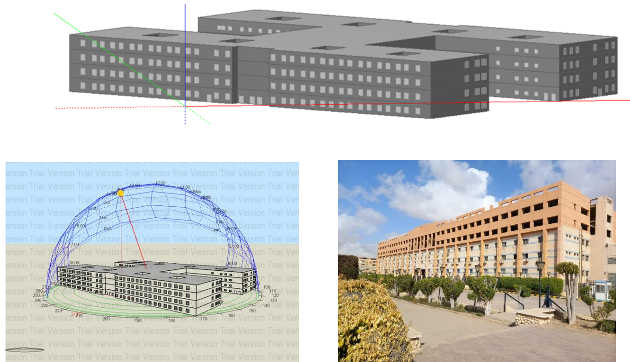
Fig.12 The base case simulation thermal model (3D Model)
