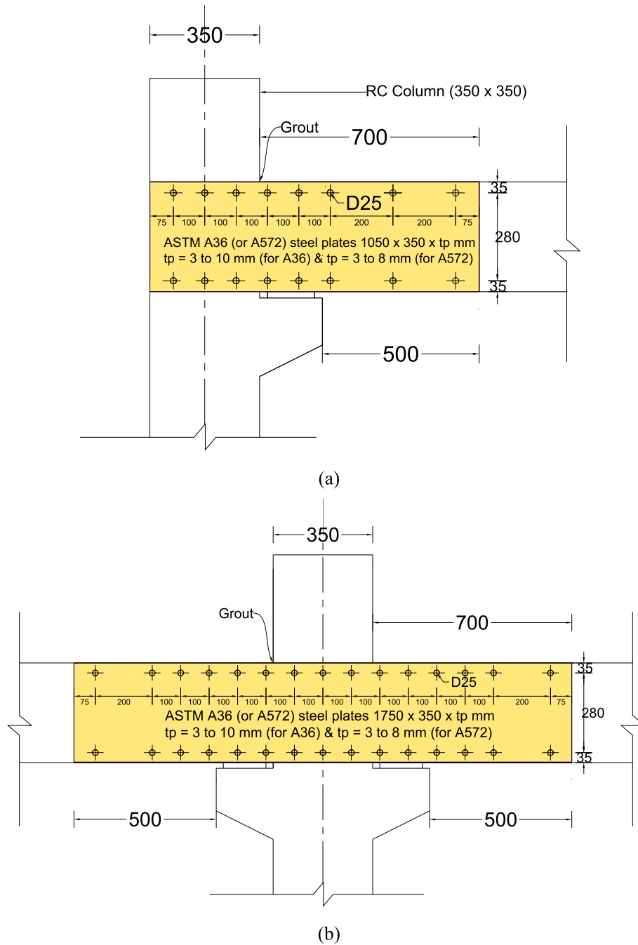
Fig. 17. Anchorage details for strengthened specimens PC-S-3-A36-FA to PC-S-10-A36-FA & PC-S-3-A572-FA to PC-S-8-A572-FA (Note: All dimensions are in mm): (a) Outer connection zone; (b) Middle connection zone.
