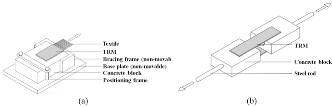
Fig. 13. TRM-to-concrete test methods [37]: (a) Single shear lap test; (b) Double shear lap test.
