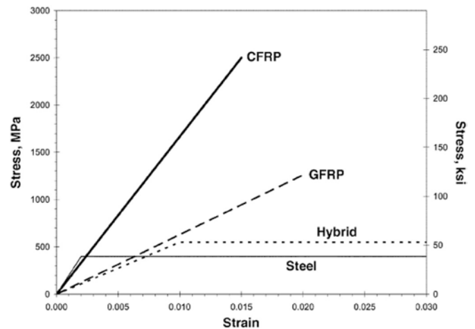
Fig. 3. Typical stress-strain curves for FRP composites [39].
