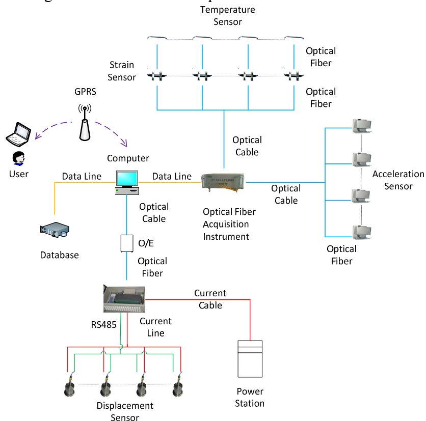
Fig.2 SHM system of Fu Sui Bridge
