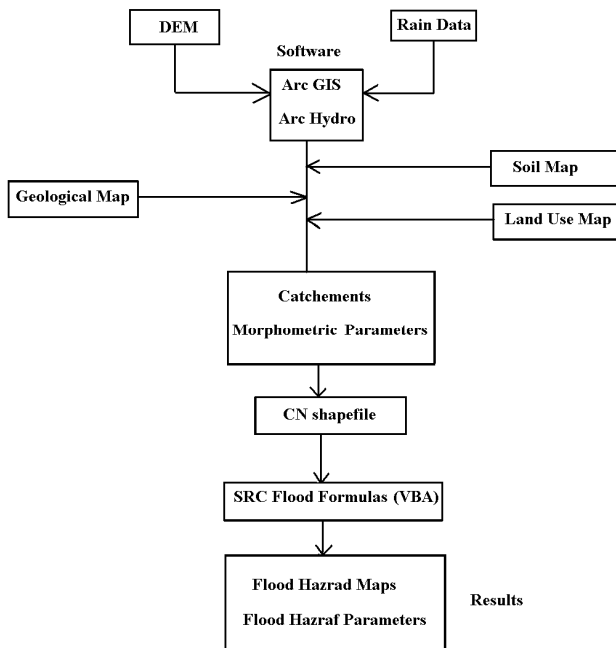
Figure 5. The developed GIS-based flood assessment methodology.
