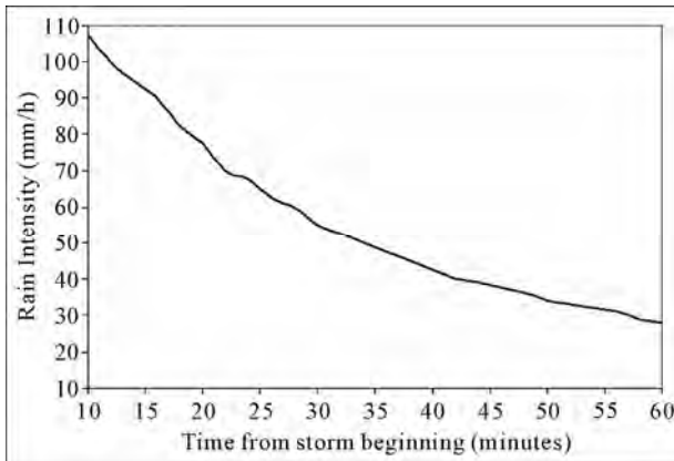
Figure 3. Rain intensity of the 1969 storm in Makkah city.
