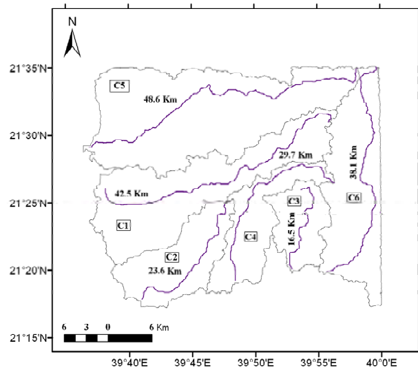
Figure 6. Catchments and their main streams.
