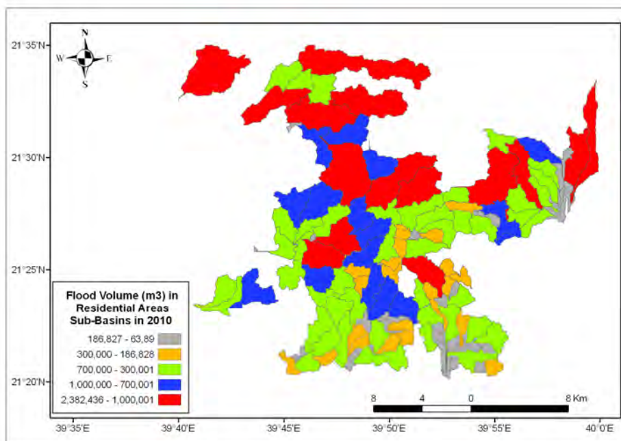
(b) Flood Volume
