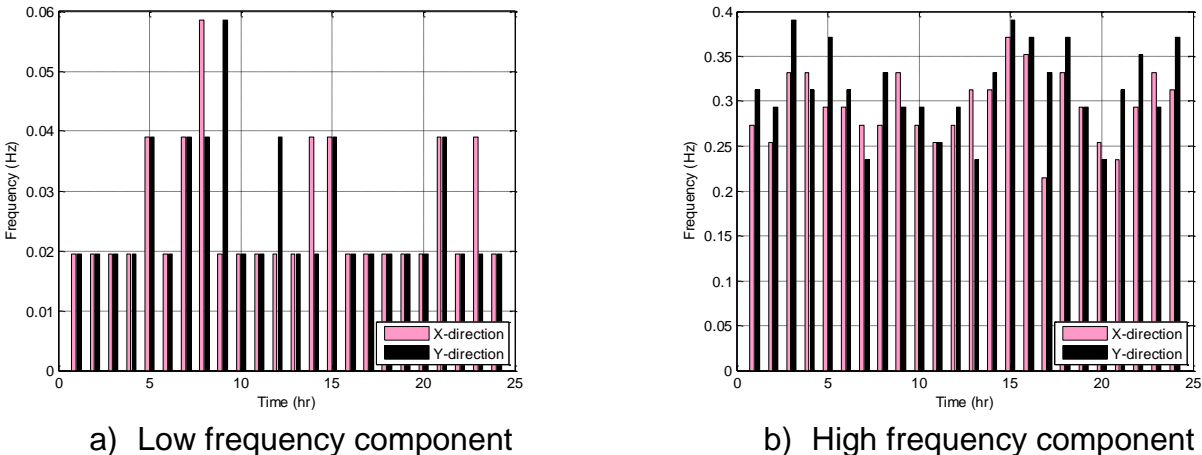
Fig. 6 Fundamental frequency components of the GPS displacement observations in the X- and Y-direction
