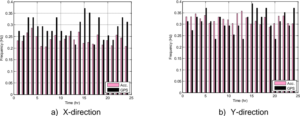
Fig. 7 Fundamental frequencies of the GPS and accelerometer acceleration observations in X- and Y-direction
