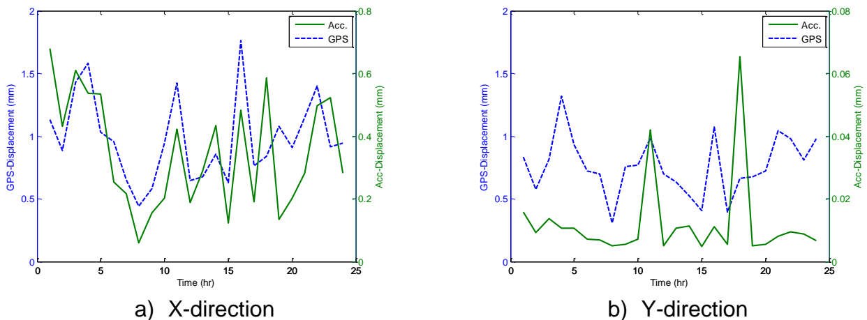
Fig. 5 Dynamic displacements components of GPS and accelerometer in the X- and Y-direction
