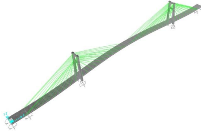
Fig. 3 Yonghe Bridge finite element first mode shape
