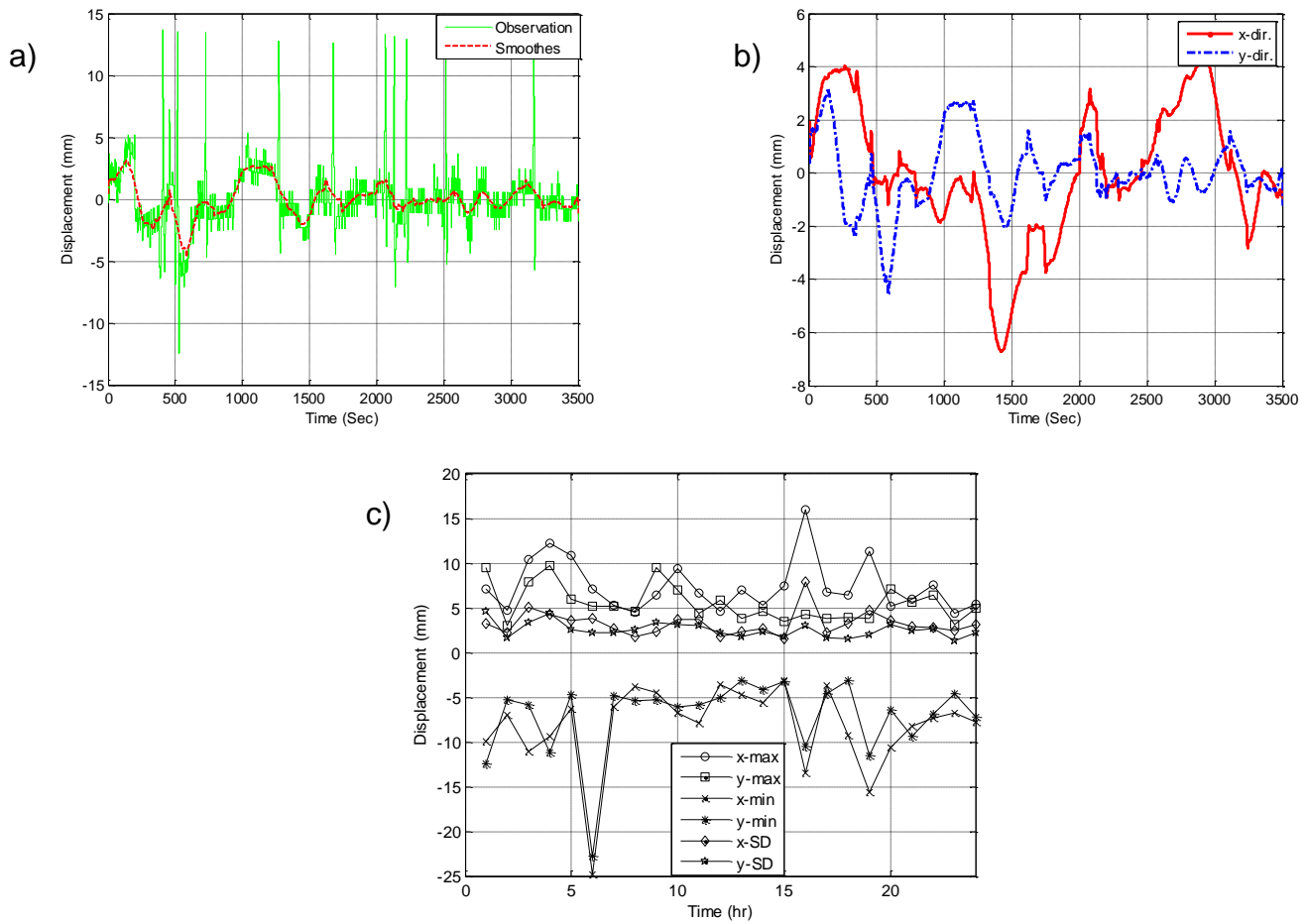
Fig. 4 GPS observations and MA smoothing filter: a) Original and smoothed GPS observations at 23:00 ; b) GPS smoothed observation of X- and Y-directions at 23:00; c) GPS displacement statistics during the observing day on January 17, 2008.
