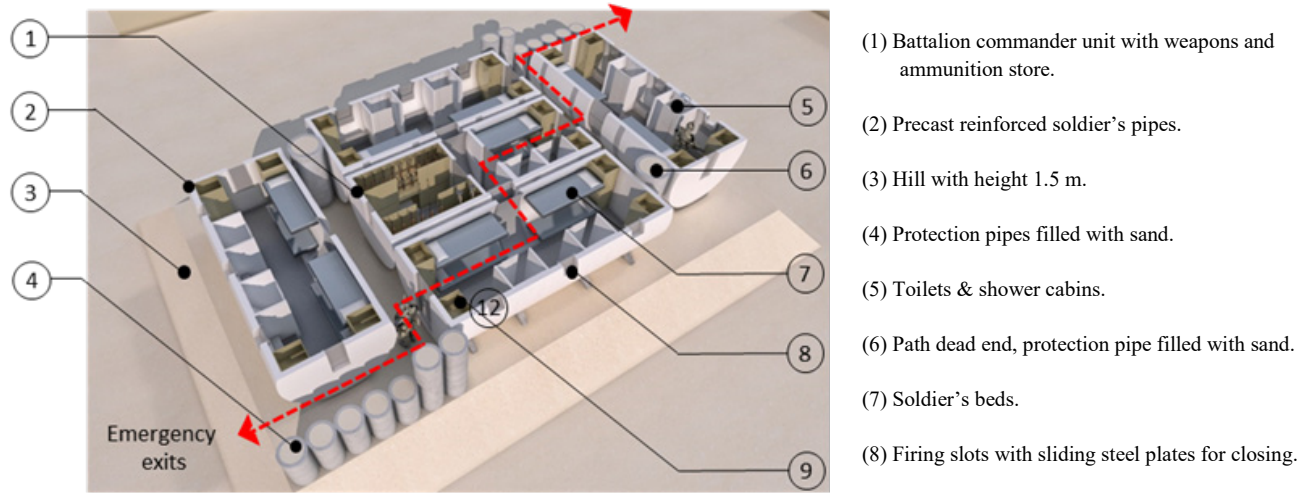
(a) The masterplan of the proposed model and its components
