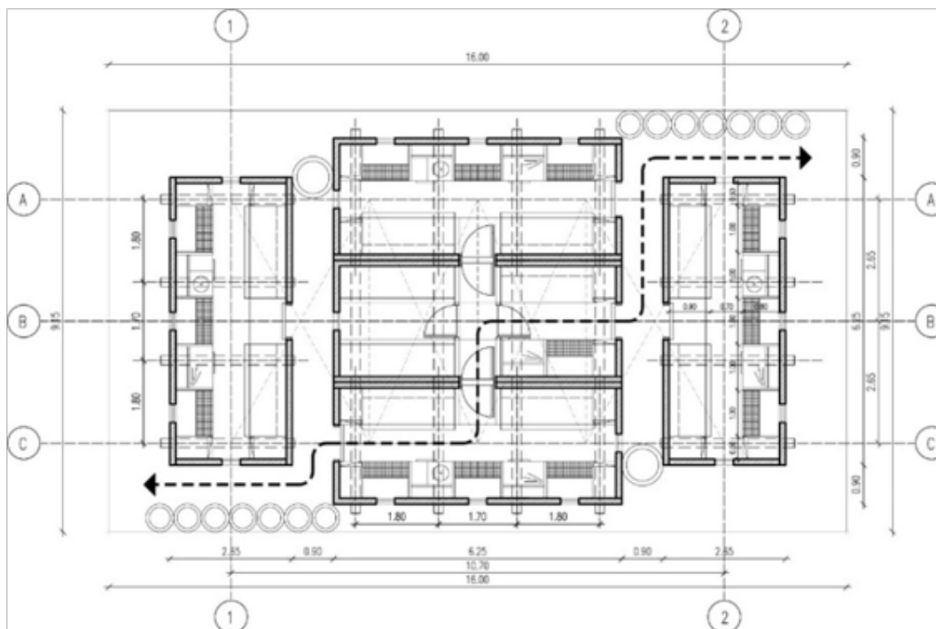
(b) The Architectural masterplan with dimension
