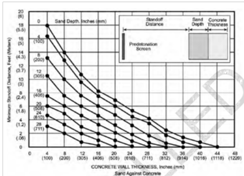
Fig. 1: Anti-tank weapon wall retrofit using sand
