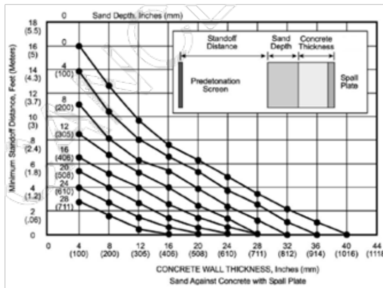
Fig. 2: Anti-tank weapon wall retrofit using sand and spall plate
