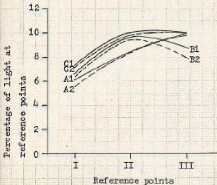
Fig. 170 Performance of window 3.00 x 1.30 Meters with reveals beveled to the interior
