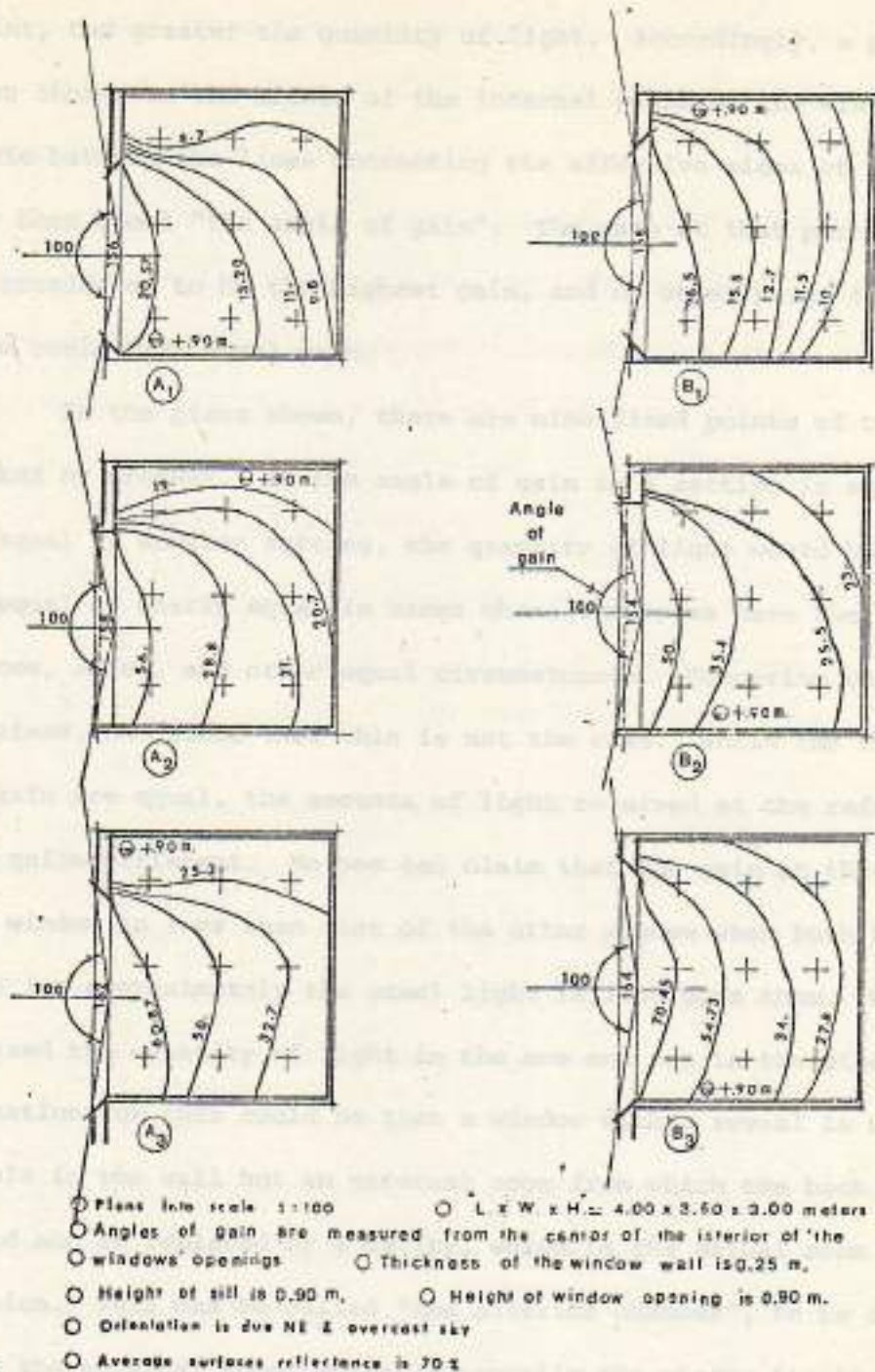
Fig 8 RELATIVE ILLUMINANCES for SEATING ROOMS with SIDE WINDOWS and DIFFERENT REVEAL SHAPES
