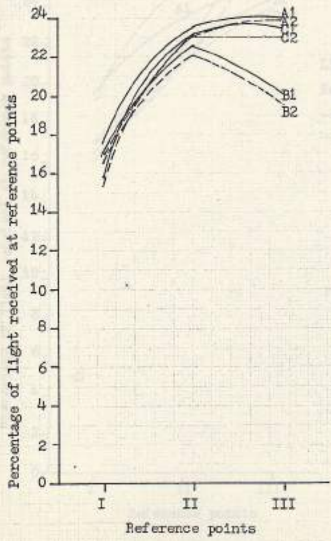
Fig. 110 Performance of window 3.60 x 1.30 Meters having square reveals
