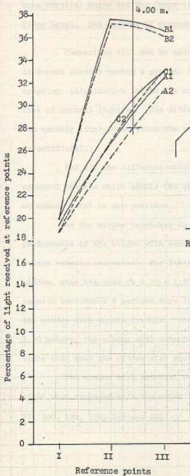
Fig. 96 Performance of window 4.00 x 1.30 Meters with reveals beveled to the exterior
