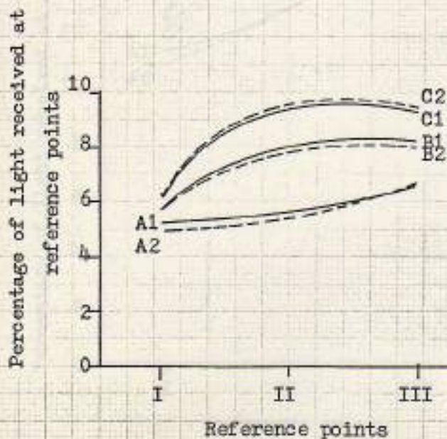
Fig. 152 Performance of window 2.40 x 1.30 Meters with reveals beveled to the interior
