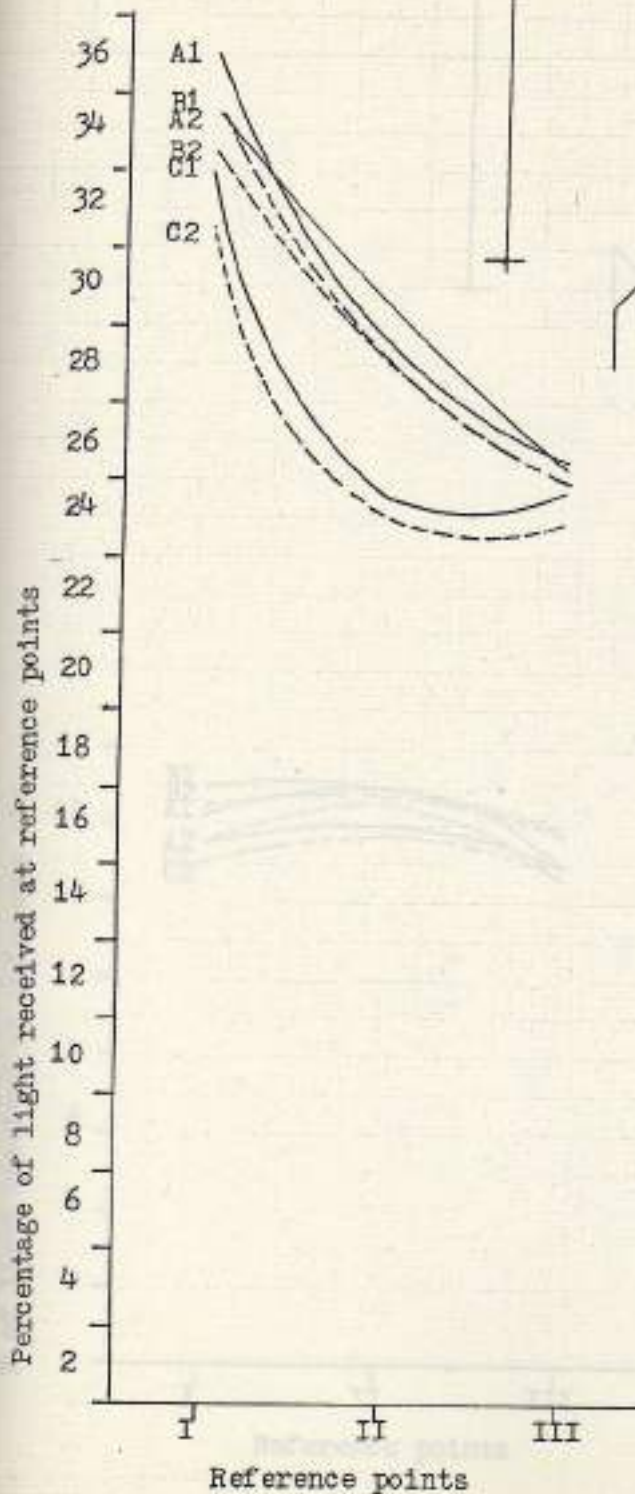
Fig. 75 Performance of window 3.60 x 1.30 Meters with square reveals
