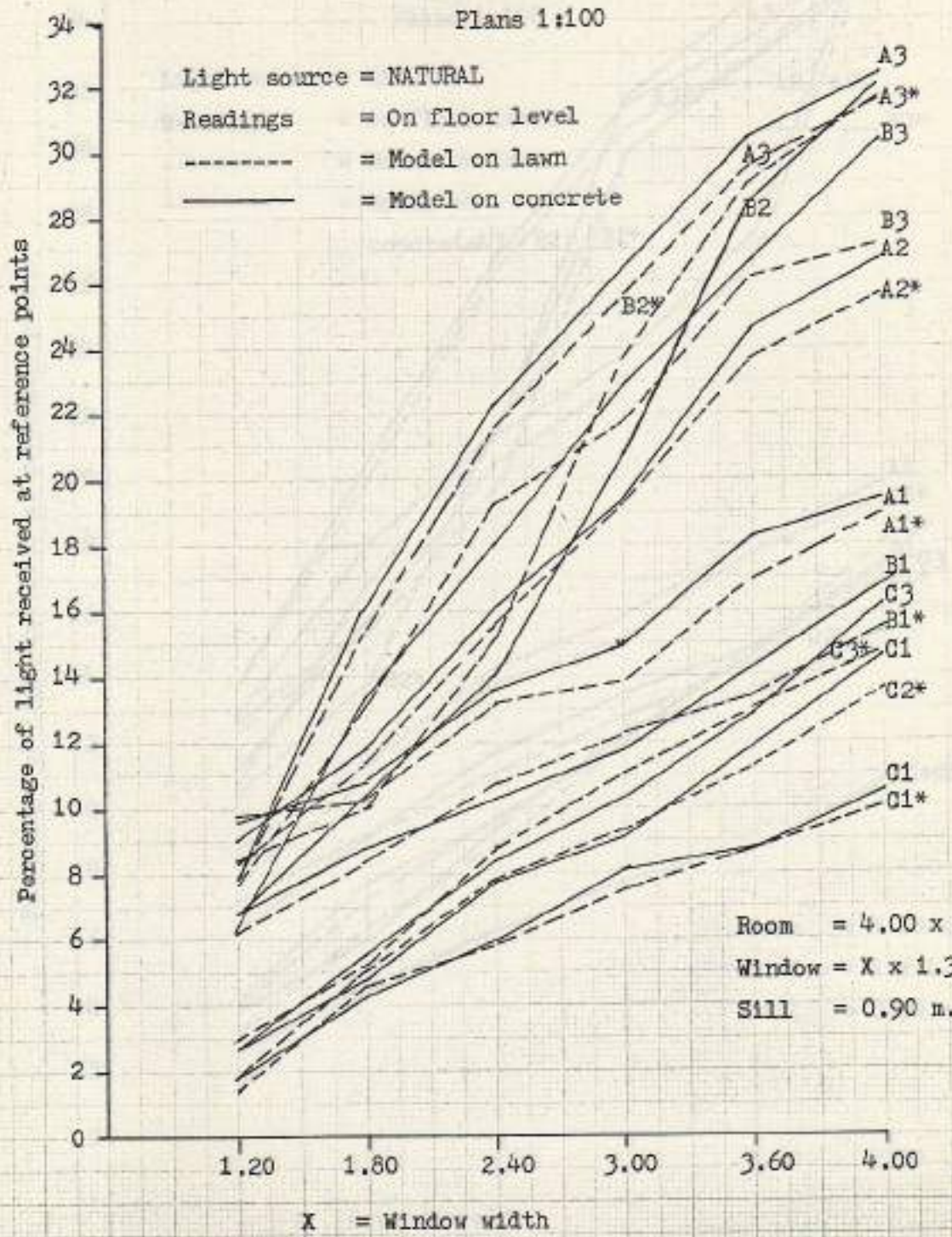
Fig. 182 Comparison between performances of windows with different reveal shapes for selected reference points
