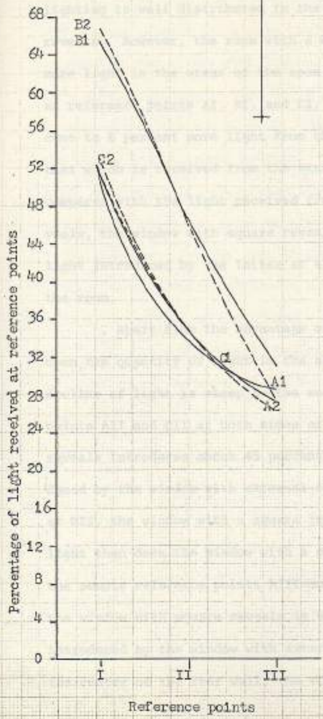
Fig. 57 Performance of window 3.60 x 1.30 Meters with reveals beveled to the exterior
