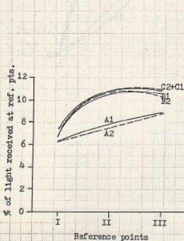
Fig. 155 Performance of window 3.00 x 1.30 Meters with reveals beveled to the interior
