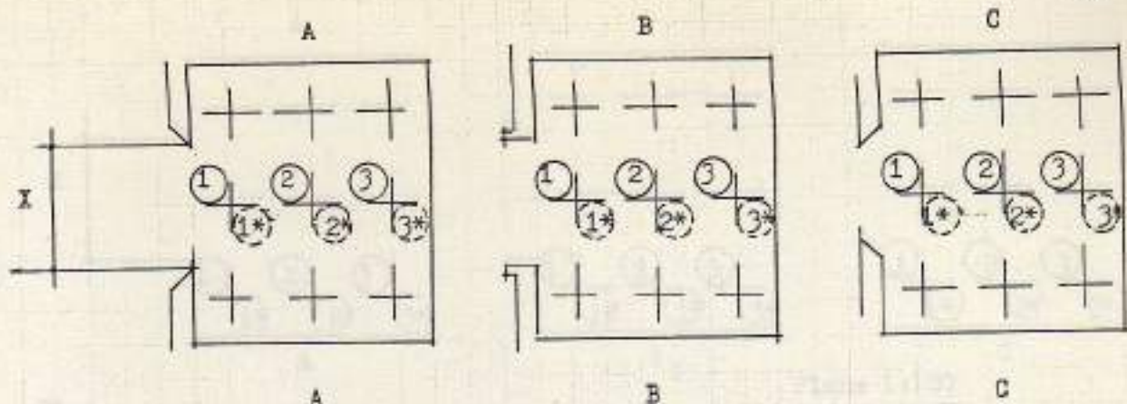
Fig. 186 Comparison between performances of windows with different reveal shapes for reference points axial to the window
