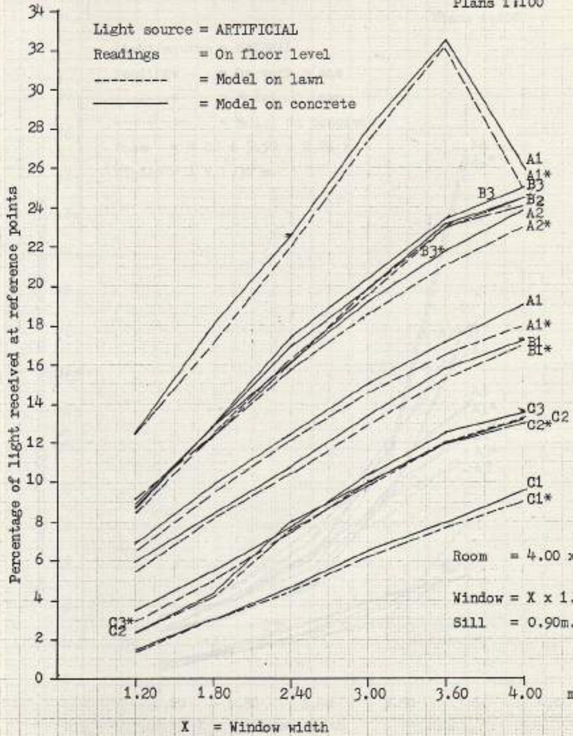
Fig. 187 Comparison between performances of windows with different reveal shapes for reference points located off-center of the windows
