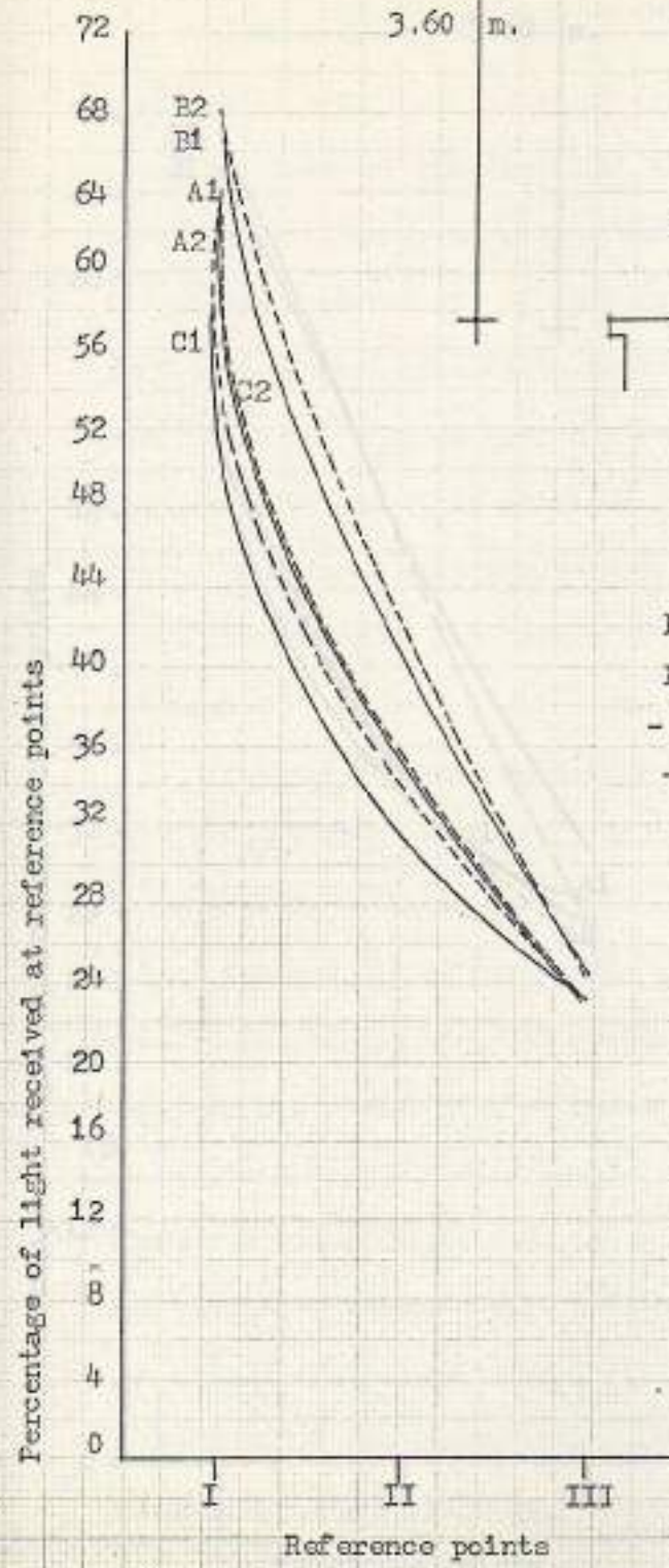
Figure 56 Performance of window 3.60 x 1.30 Meters with square reveals
