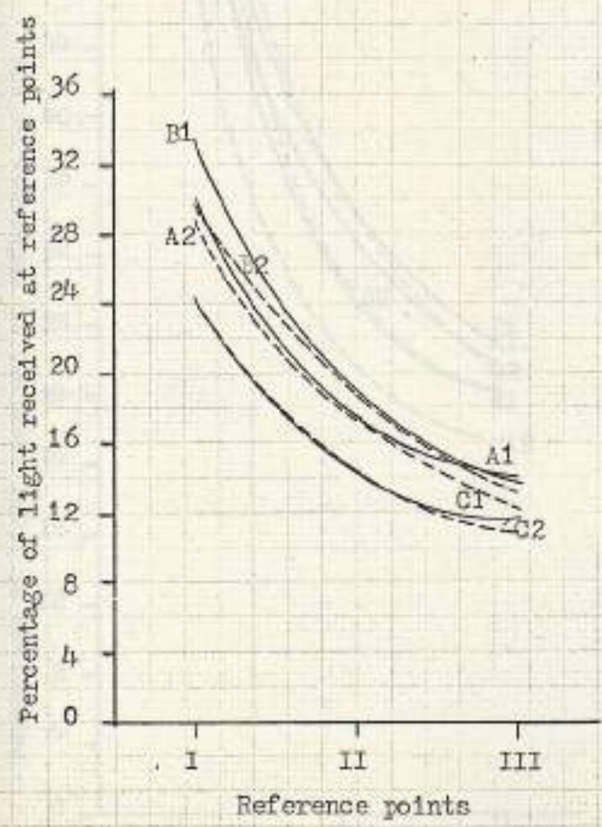
Fig. 58 Performance of window 4.00 x 1.30 Meters with reveals beveled to the interior
