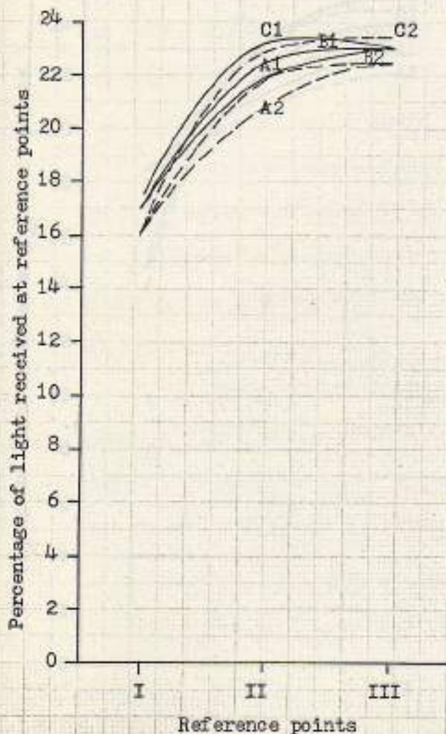
Fig. 174 Performance of window 3.60 x 1.30 Meters with square reveals
