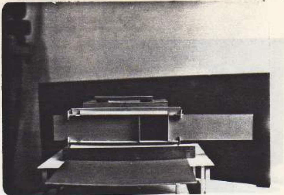
Figure 37 Model of the room having a window with square reveals and located at one side of the side wall (Window reveals are extended 0.12 Meters beyond the wall thickness).
