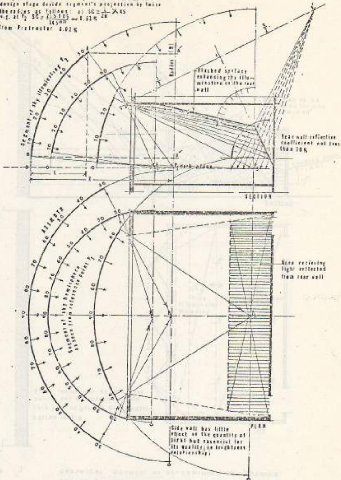
Fig 2 GEOMETRICAL METHOD of DESIGNING ROOM SHAPE for READING ROOMS with SIDE WINDOWS and NO EXTERNALLY REFLECTED COMPONENT ETC
