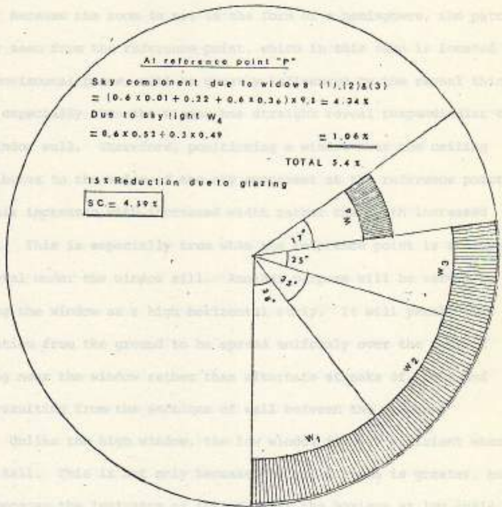
Fig 14 Method of calculating the sky component from example in fig 13 by the aid of the proposed protractor for "CIE" overcast sky
