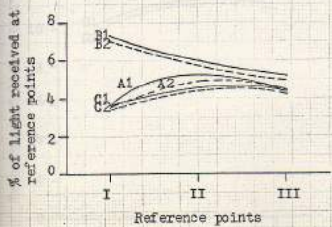
Fig. 64 Performance of window 1.80 x 1.30 Meters having reveals beveled to the interior
