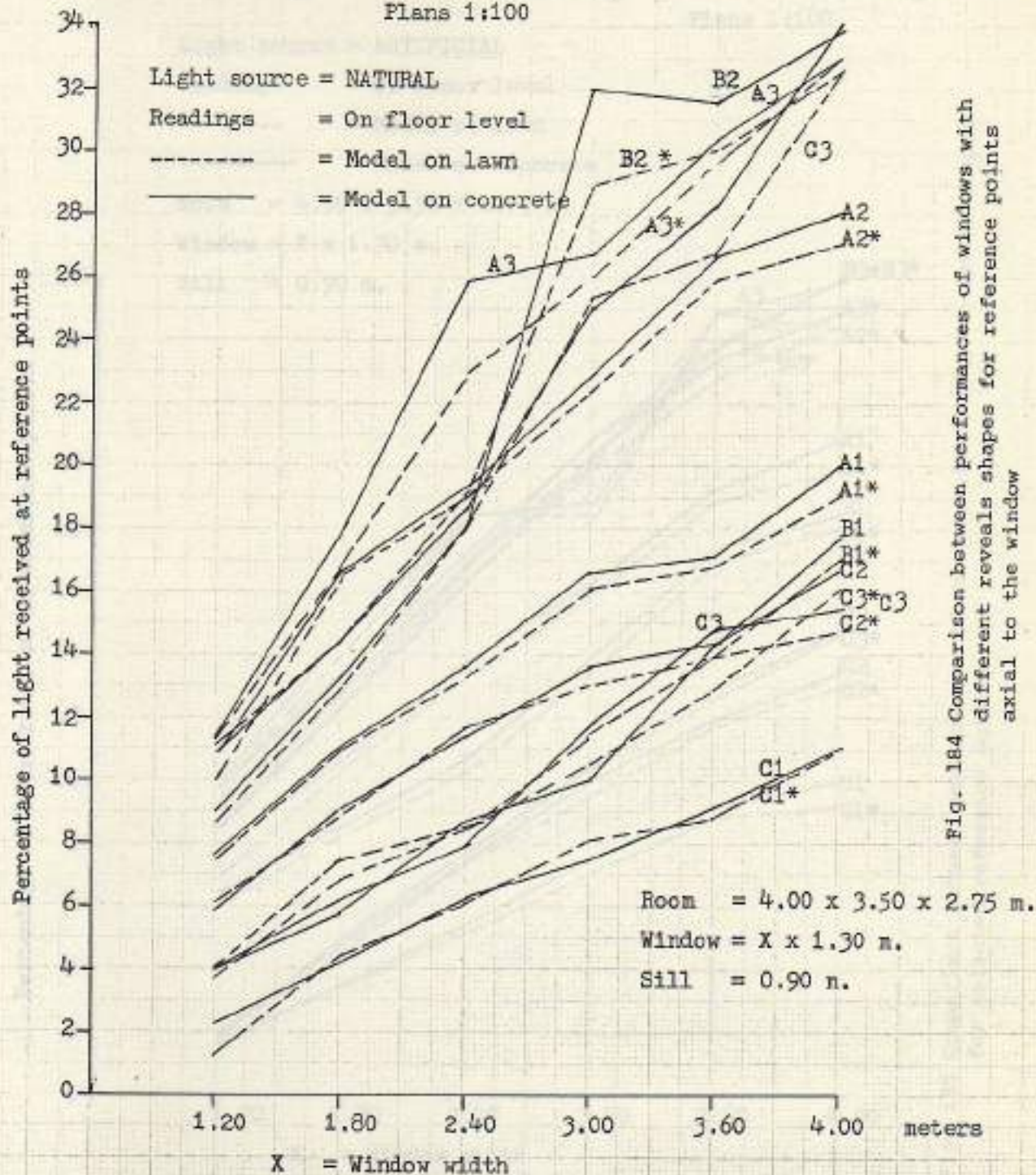
Plans 1:100
