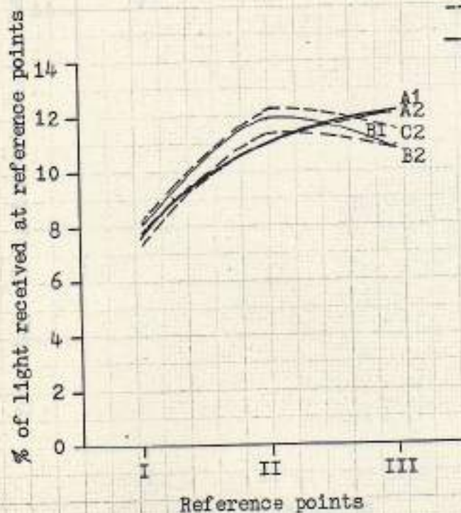
Fig. 173 Performance of window 3.60 x 1.30 Meters with reveals beveled to the interior
