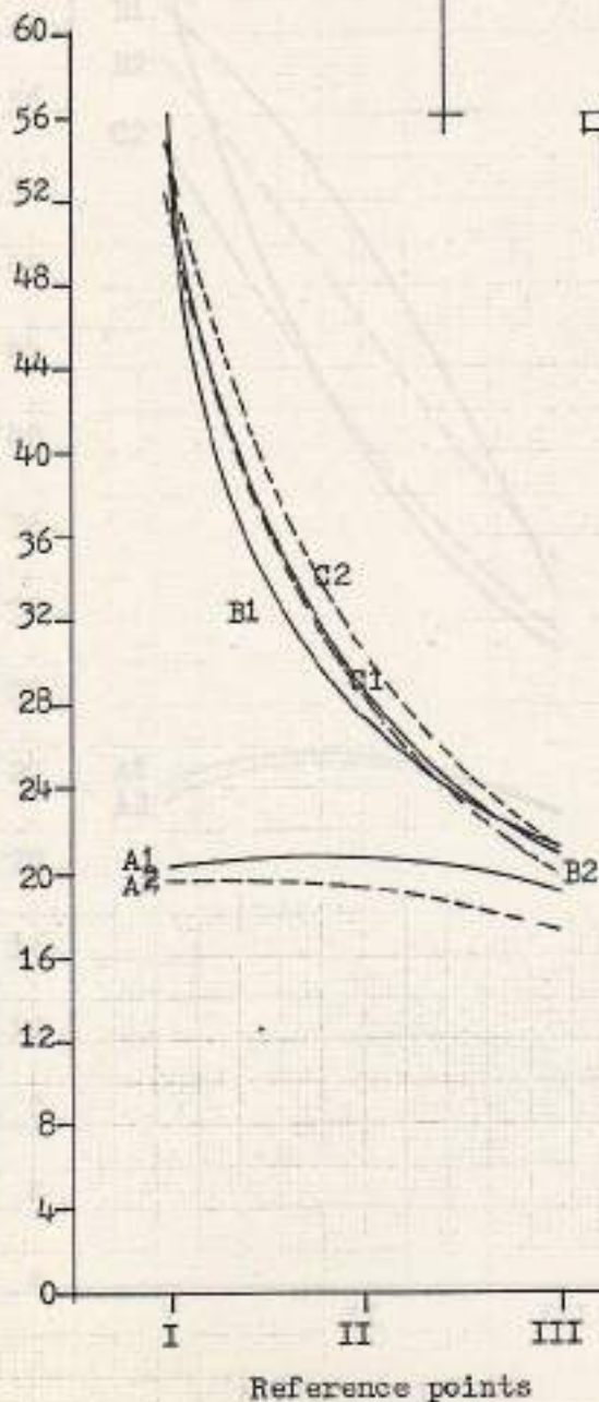
Fig. 126 Performance of window 3.00 x 1.30 Meters having square reveals located at one side of the wall
