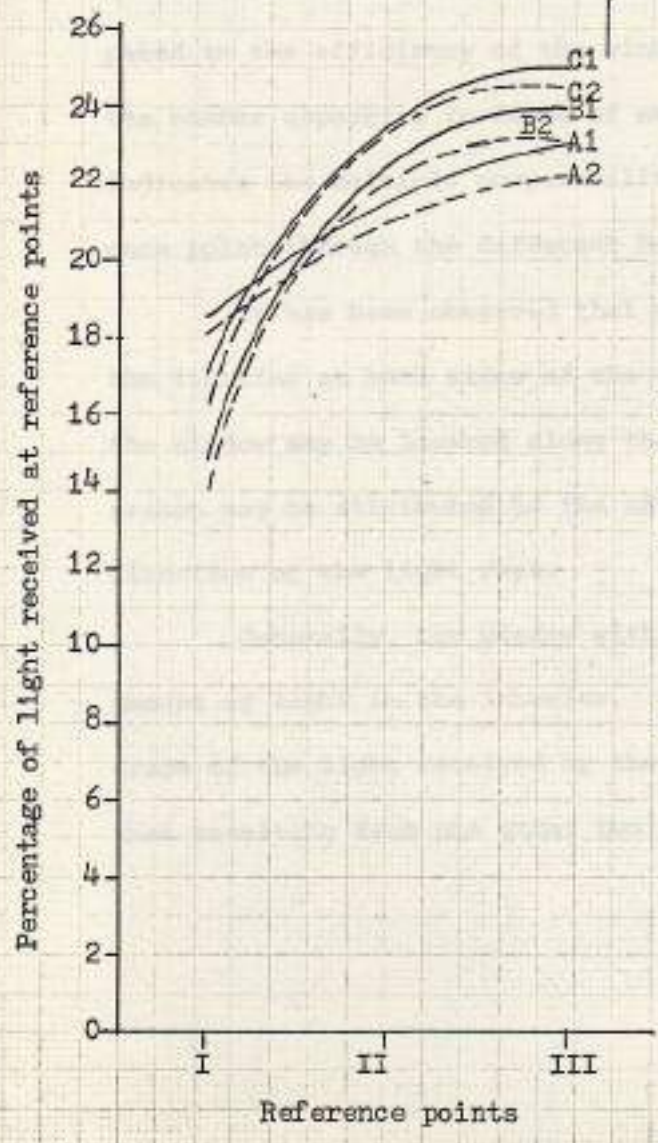
Fig. 175 Performance of window 3.60 x 1.30 Meters with reveals beveled to the exterior
