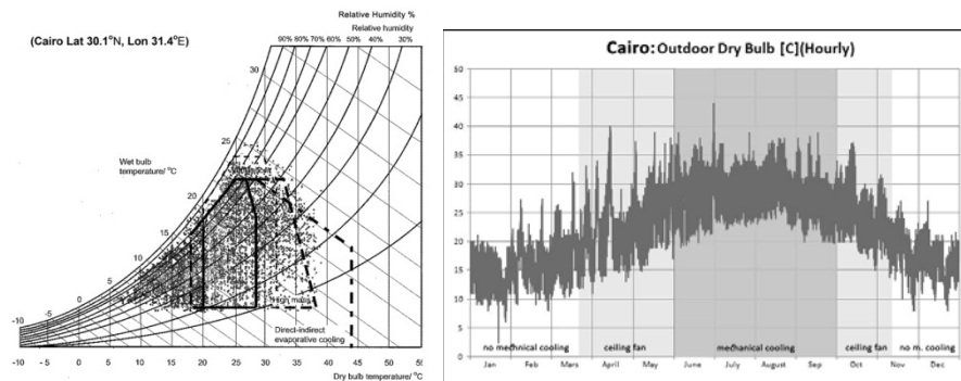
Figure 4.10a. Psychrometric chart analysis for Cairo Figure 4.10b. Operational periods defined using simulations
