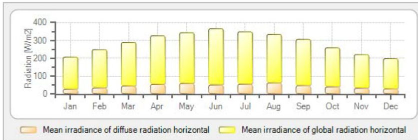
Figure AA1 Weather Data for Alexandria (METEONORM)
