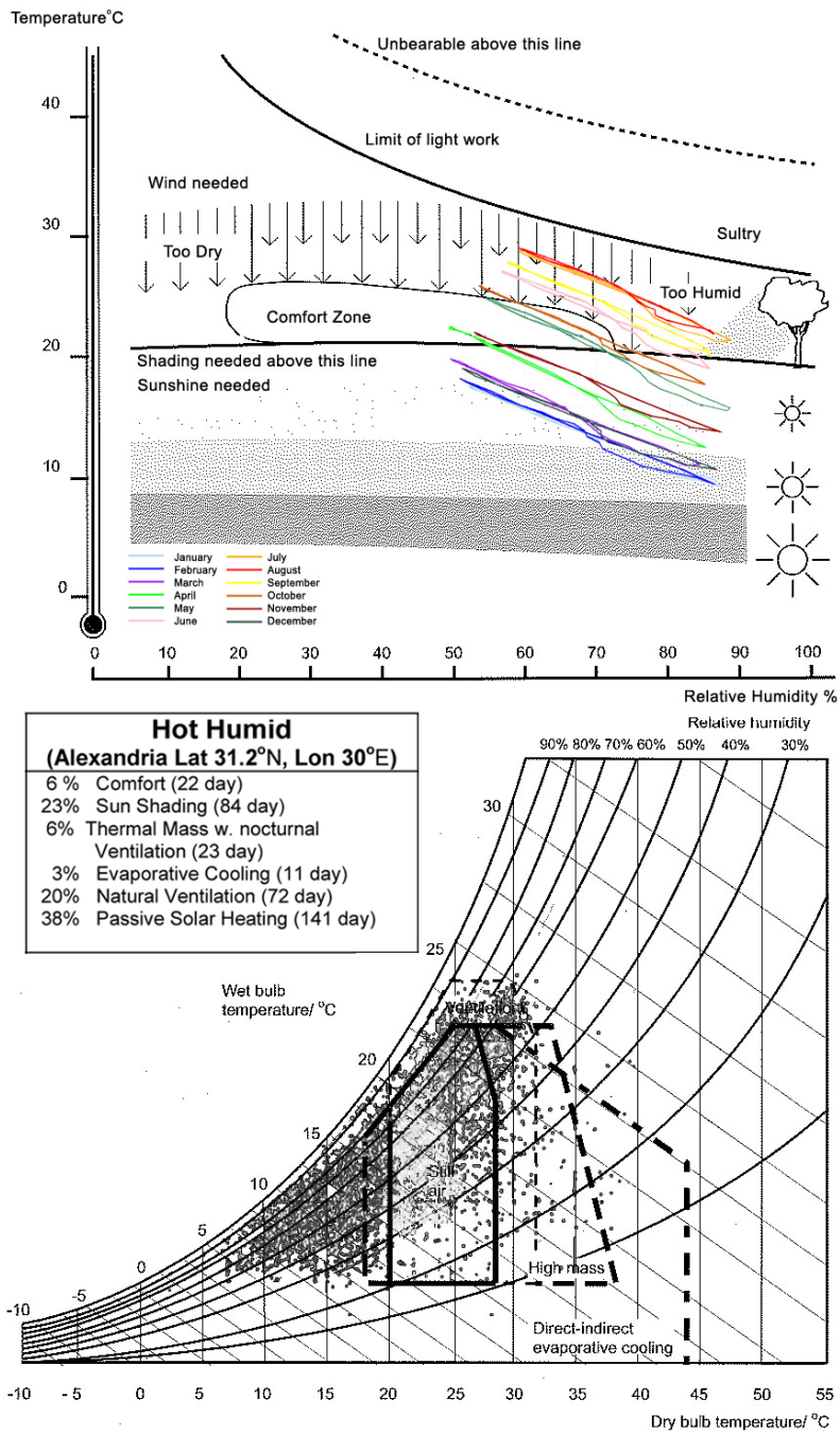
Figure 2.9 Psychrometric chart analysis and the corresponding passive design strategies for Alexandria (Climate Consultant 5 see Appendix A)
