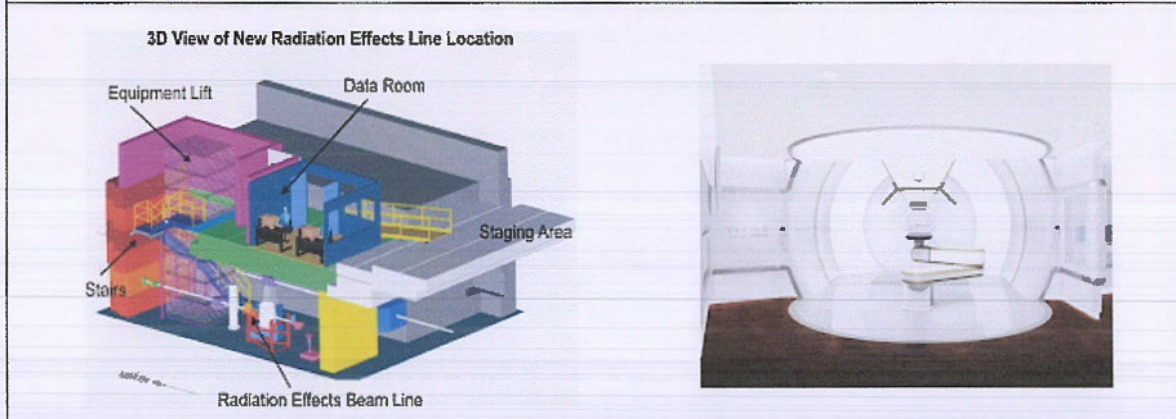
Figure 6: Data Room is Located Directly Above the Radiation Effects Facility
