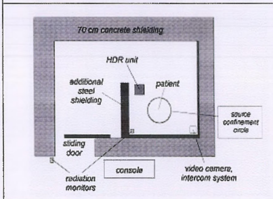
Figure 7: HDR Room Design (Example)
