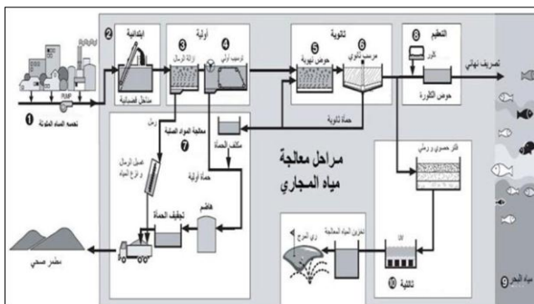
Fig(1): Wastewater treatment stages applied in Centralized system in Egypt - www.hcww.com.eg
