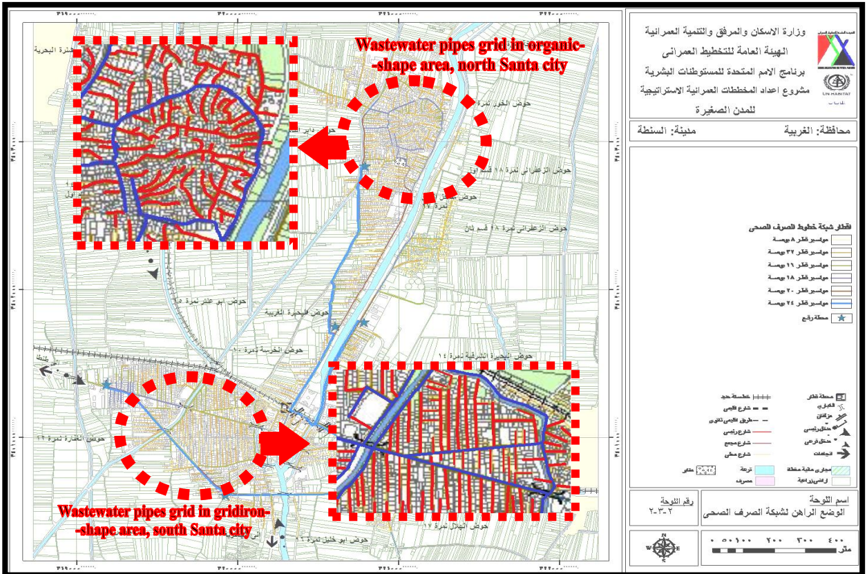
Fig(8): Comparing grid lines in both organic and gridiron-shape areas in Alsanta village, Gharbeya, Egypt
