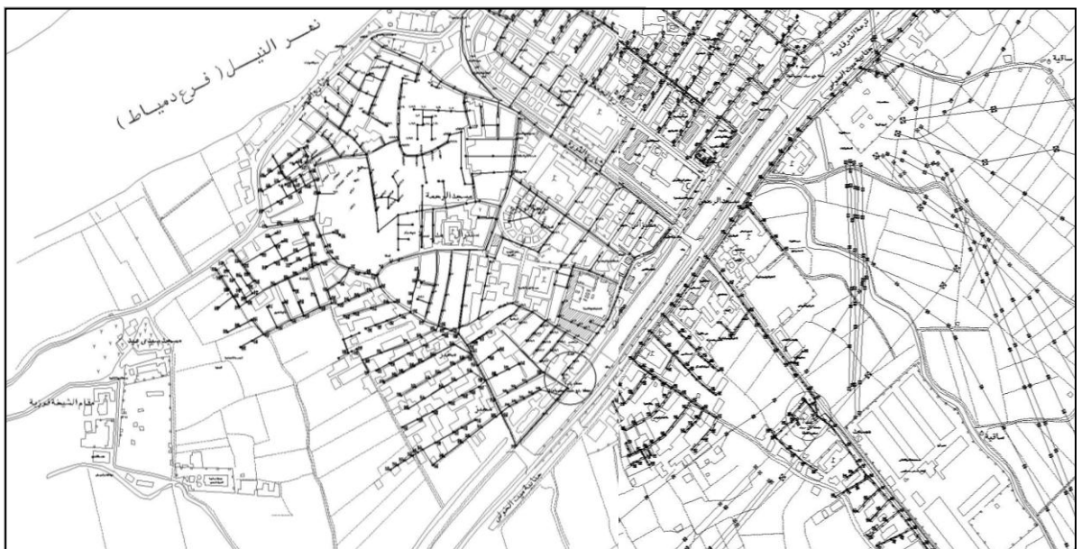
Fig(13): Wastewater grid in Al-Zarka city, Damietta- Source: General Organization for Urban Planning (GOPP).
