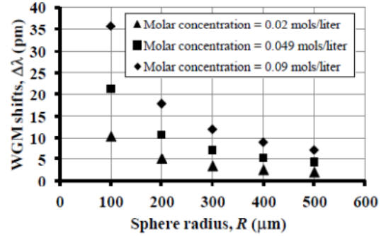
Figure 4. Measured WGM shift dependence on the sphere size
