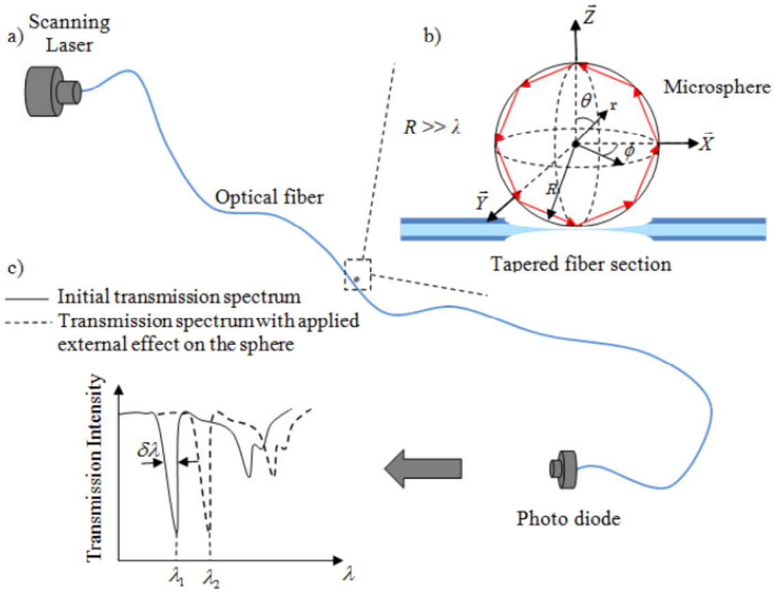
Figure 1: a) Typical WGM sensor configuration, b) Ray optics model of light traveling inside sphere for one round trip, c) Transmission spectrum for a spherical resonator (Ali).
