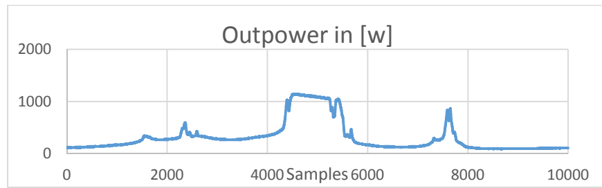
Figure 4: The output response of output AC power from the drive
