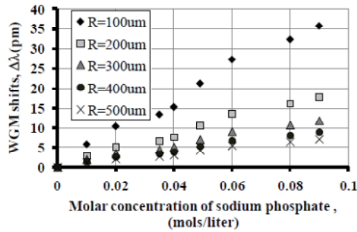
Figure 3. Measured WGM shift dependence on the sodium phosphate concentrations
