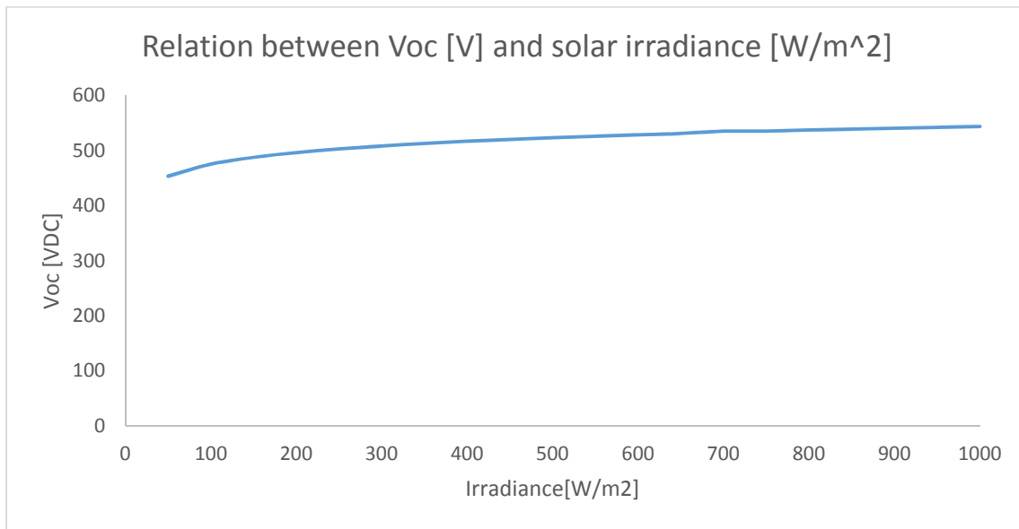
Figure 3: Relation between Voc [V] and solar irradiance [W/m 2 ]
