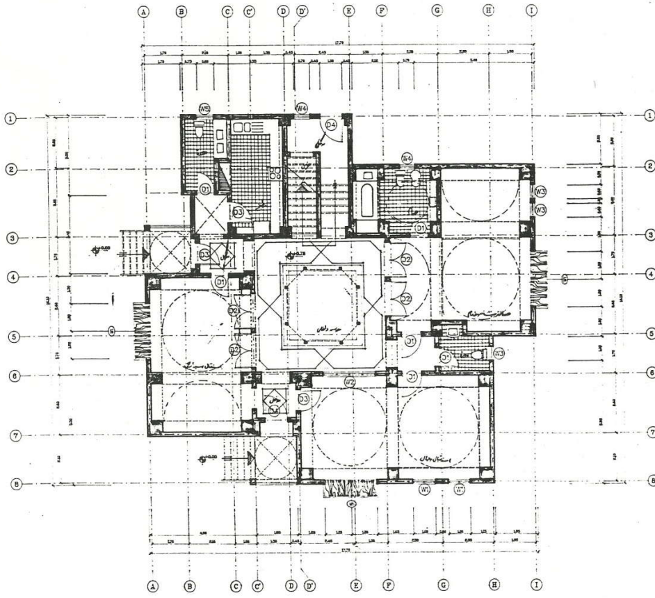
⊕ GROUND FLOOR PLAN SCALE
