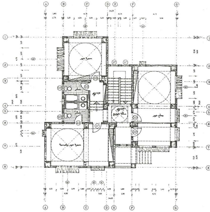
① FIRST FLOOR PLAN SCALE 1/100
